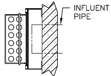
RAILS MOUNTED IN RECTANGULAR BASIN
