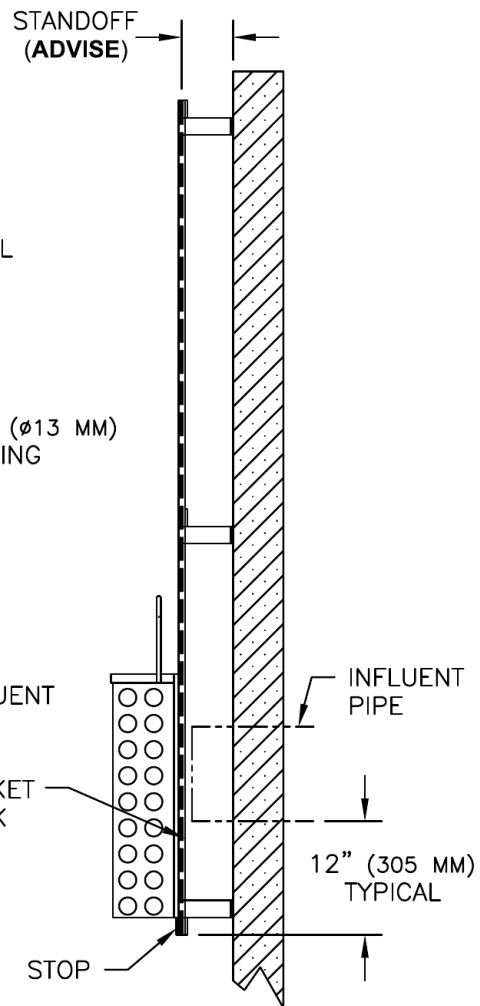
RAILS MOUNTED IN RECTANGULAR BASIN
