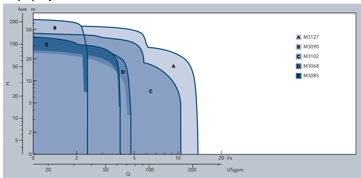
Pump capacity, 60 Hz
